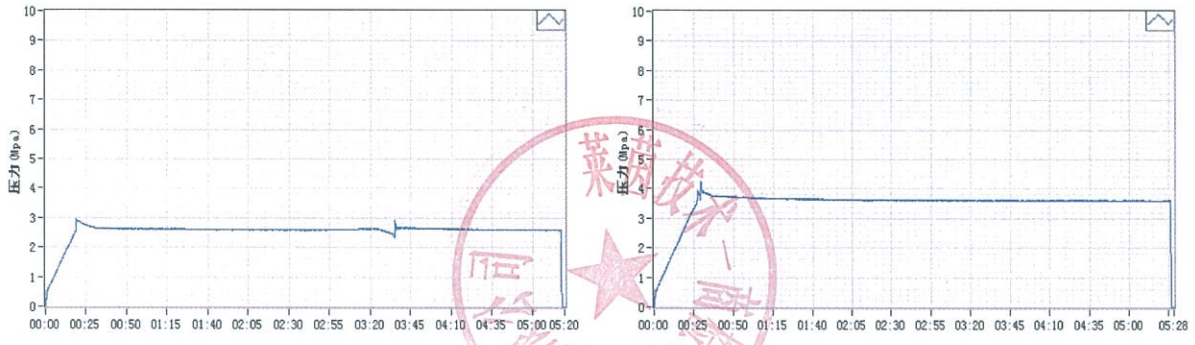
Pic. 05 : 25bar Withstand test curve Pic. 06 : 35bar Withstand test curve
