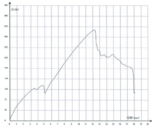
Pic. 08 : Drawing Force Testing Curve
